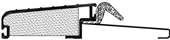
OUTSWING THRESHOLD (Aluminum Bumper Style)
