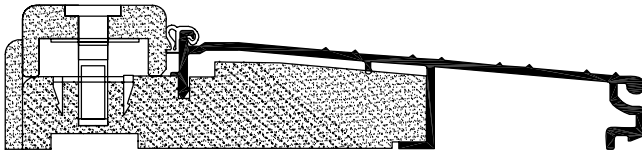
THRESHOLD (Adjustable Type, Aluminum)
